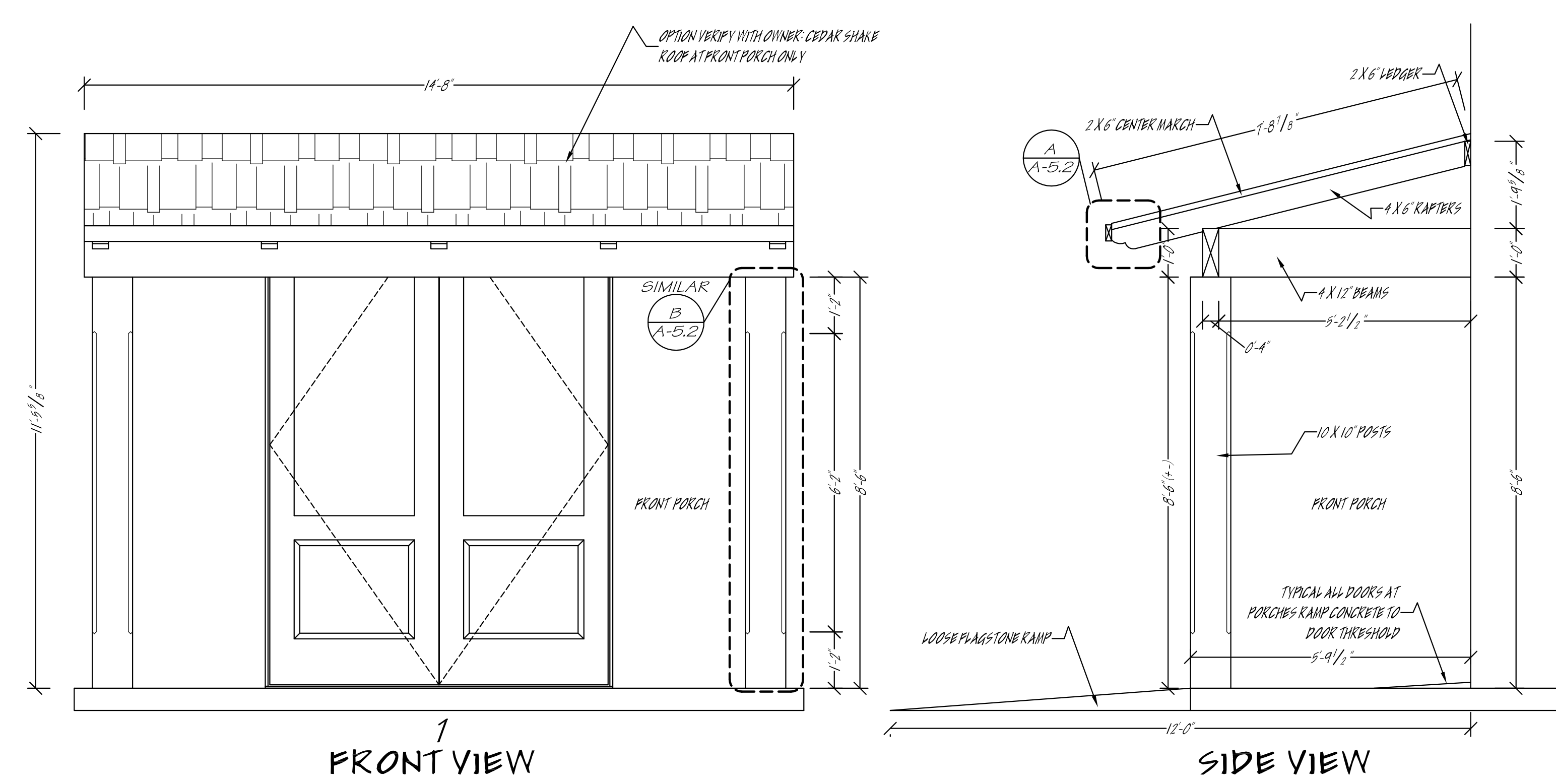
FRONT ENTRY DETAILS 12'-1'0"
